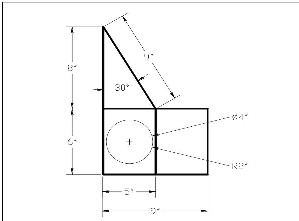
Figure 2.21: Linear Dimension
