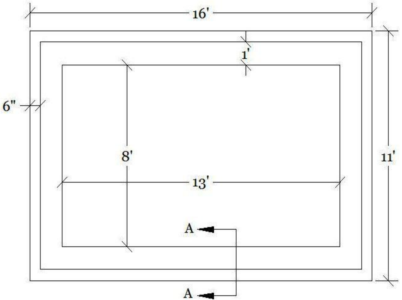
Figure 6.1: Plan of the underground water reservoir
