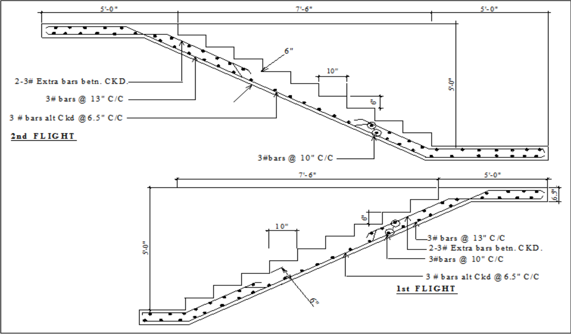
Figure 4.4: Reinforcement detailing of stair
