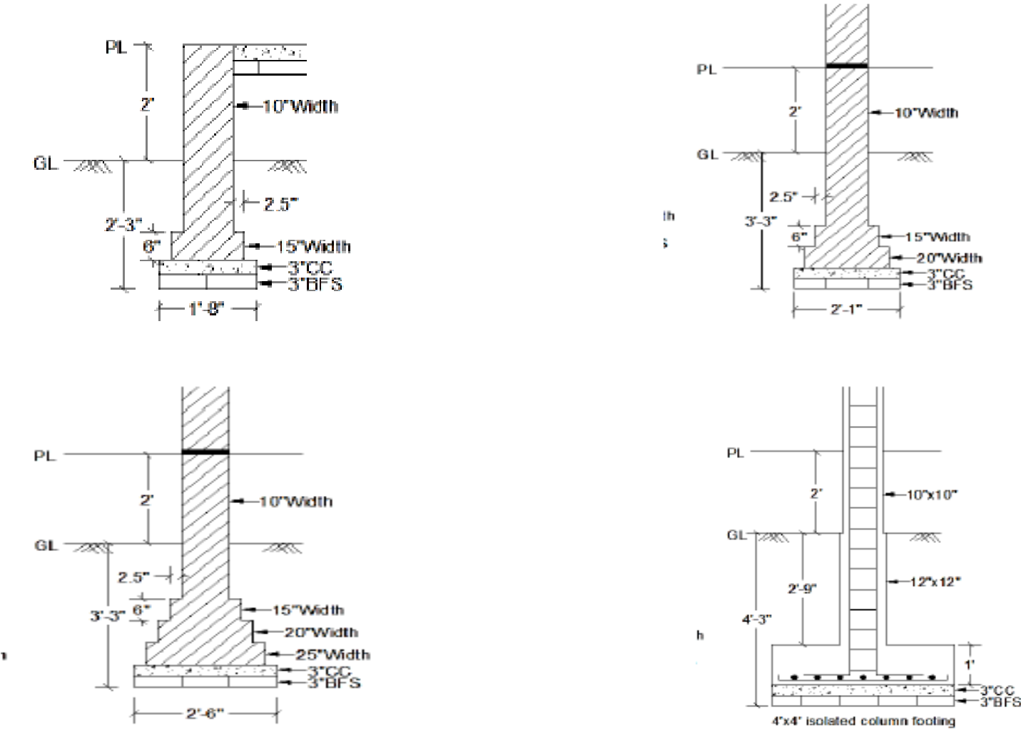
Figure 4.1: Wall Footing and Column Footing
