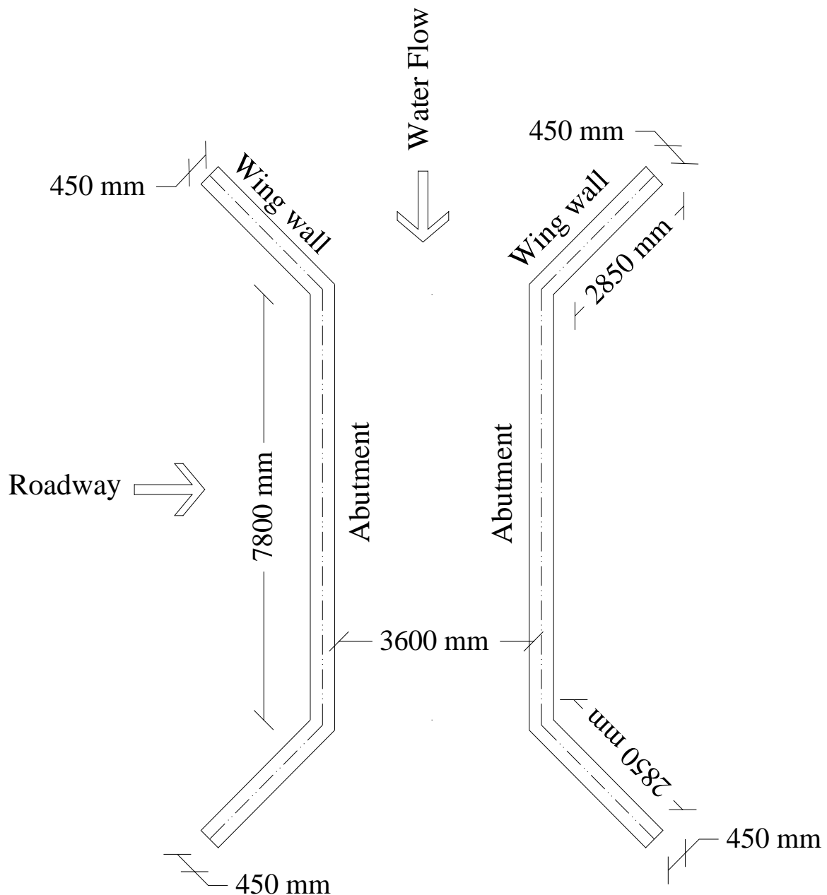
Figure 5.1: Plan of the Culvert.
