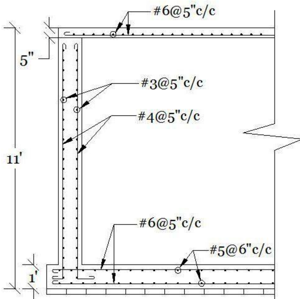
Figure 6.2: Section A-A
